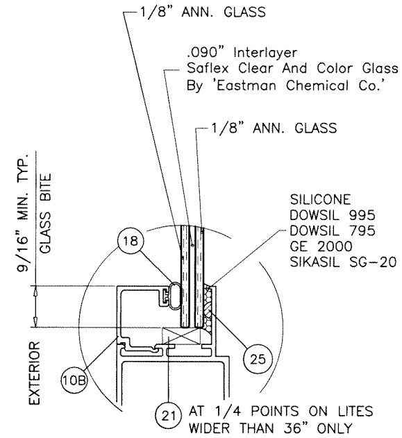
GLASS TYPE 'C' 5/16" OVERALL LAM. GLASS
